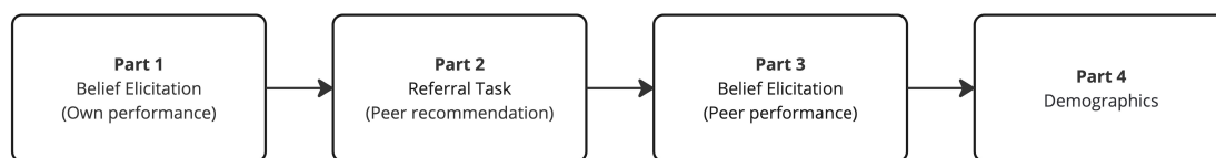
Figure 2: Experiment Overview
